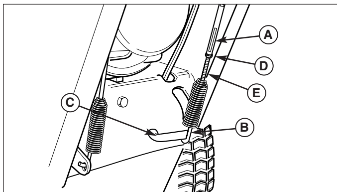
Figure 19. Skruvens remspänning
